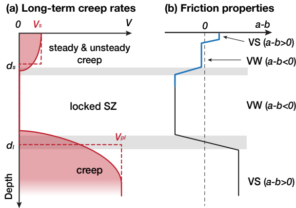
Figure 12. Simple models for fault slip and rheology of the SSAF. (a) Creep on the fault occurs above and below the interseismically locked, seismogenic zone (SZ). The surface creep consists of steady creep and unsteady creep events, above the depth d_s ; the average creep rate at the surface, V_s , is directly determined by d_s , the effective locking depth of the fault, d_l , and the long-term plate-loading rate, V_{pl} . The solid line indicates a stress-controlled crack model of deep creep that has similar stressing on the shallow fault, compared to the dislocation model (dashed line). (b) The shallow unsteady and steady fault creep can result from velocity-strengthening (VS, a - b > 0 ) and mildly velocity-weakening (VW, a - b < 0 and a - b \sim 0 ) frictional properties on top of the velocity-weakening (VW) seismogenic zone and deeper VS fault extension. Horizontal bars in gray indicate locked-creeping transition zones. We impose fault slip rates in regions marked in black and solve for the fault stress, slip rate, and state variables in regions marked in blue.
