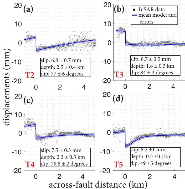
Figure 10. Results of inversions of surface displacements for the amplitude, depth, and dip of shallow creep. Panels a-d show profiles of fault-parallel displacements at several locations along the fault trace (see white circles in Figure 7b). Black dots denote InSAR data, and blue lines denote the best fitting models. Shaded blue areas denote the model uncertainties. The respective model parameters are presented below each model.
