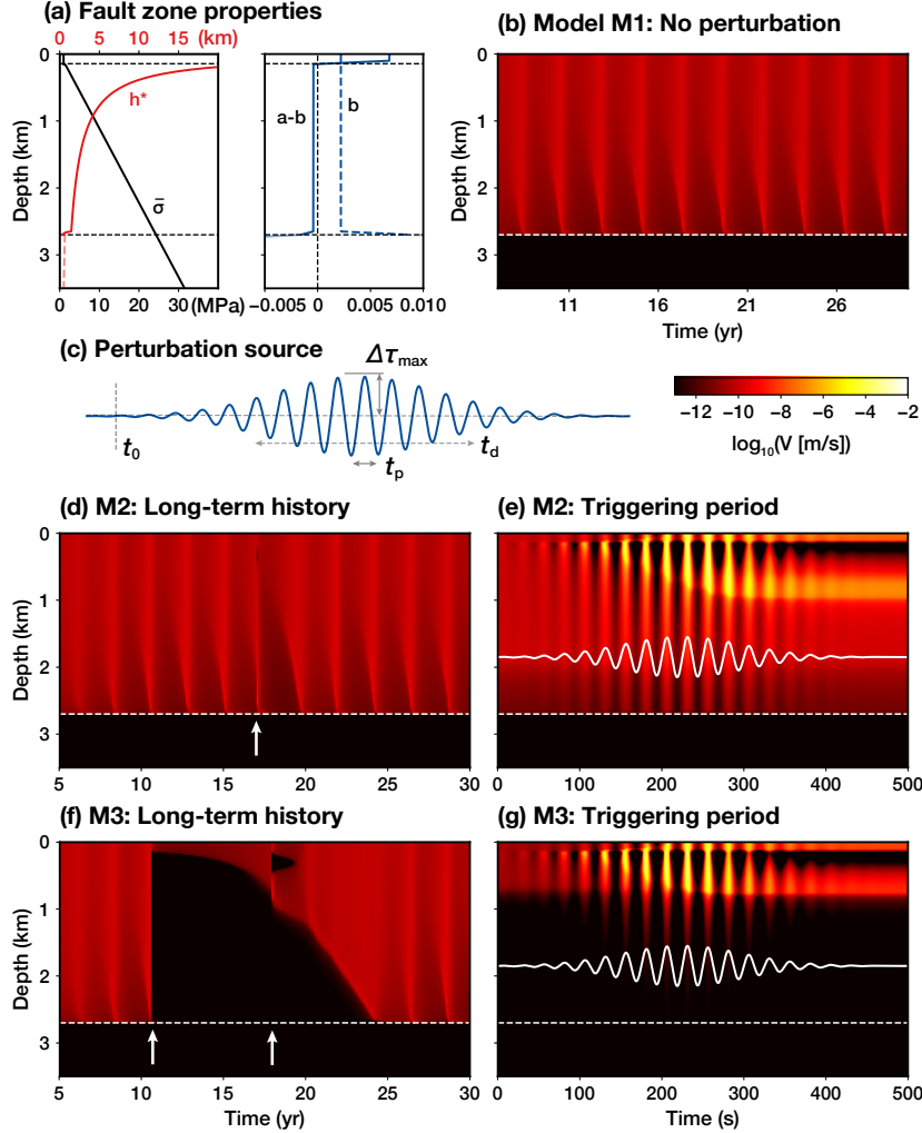
Figure 13. Depth-dependent fault properties and responses to dynamic perturbations. (a) Depth-profiles of (left) the effective normal stress, \bar{\sigma} and locally estimated nucleation size of VW fault areas, h^* (solid red line; dashed line indicates the deeper seismogenic zone) and (right) rate-and-state frictional parameters ( a - b ) (solid blue line) and b (dashed blue line). (b) The time evolution of logarithmic slip rates on the fault for the case without perturbations. (c) The temporal function of the applied dynamic stress perturbation, parameterized by the onset time, t_0 , maximum dynamic Coulomb stress change, \Delta\tau_{max} , characteristic period, t_p , and duration, t_d . The responses of these shallow fault areas to dynamic perturbations are depth- and history-dependent. The time evolution of slip rates in these perturbed cases are shown for: (d-e) a single dynamic perturbation ( \Delta\tau_{max}=69 kPa) and (f-g) two consecutive dynamic perturbations ( \Delta\tau_{max}=85 and 74 kPa, respectively). The left column (d and f) shows long-term slip history; the right column (e and g) shows the triggering period. White arrows mark the time of applied dynamic stress perturbations. The waveforms (white) in (g) are drawn to illustrate stress changes at corresponding time.
