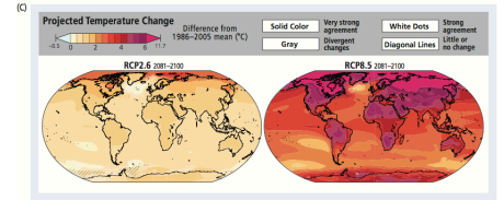
Figure SPM.4 | Observed and projected changes in annual average surface temperature. This figure informs understanding of climate-related risks in the WGI/AR5. It illustrates temperature change observed to date and projected warming under continued high emissions and under ambitious mitigation.
