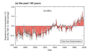
Variations of the Earth's surface temperature for:
