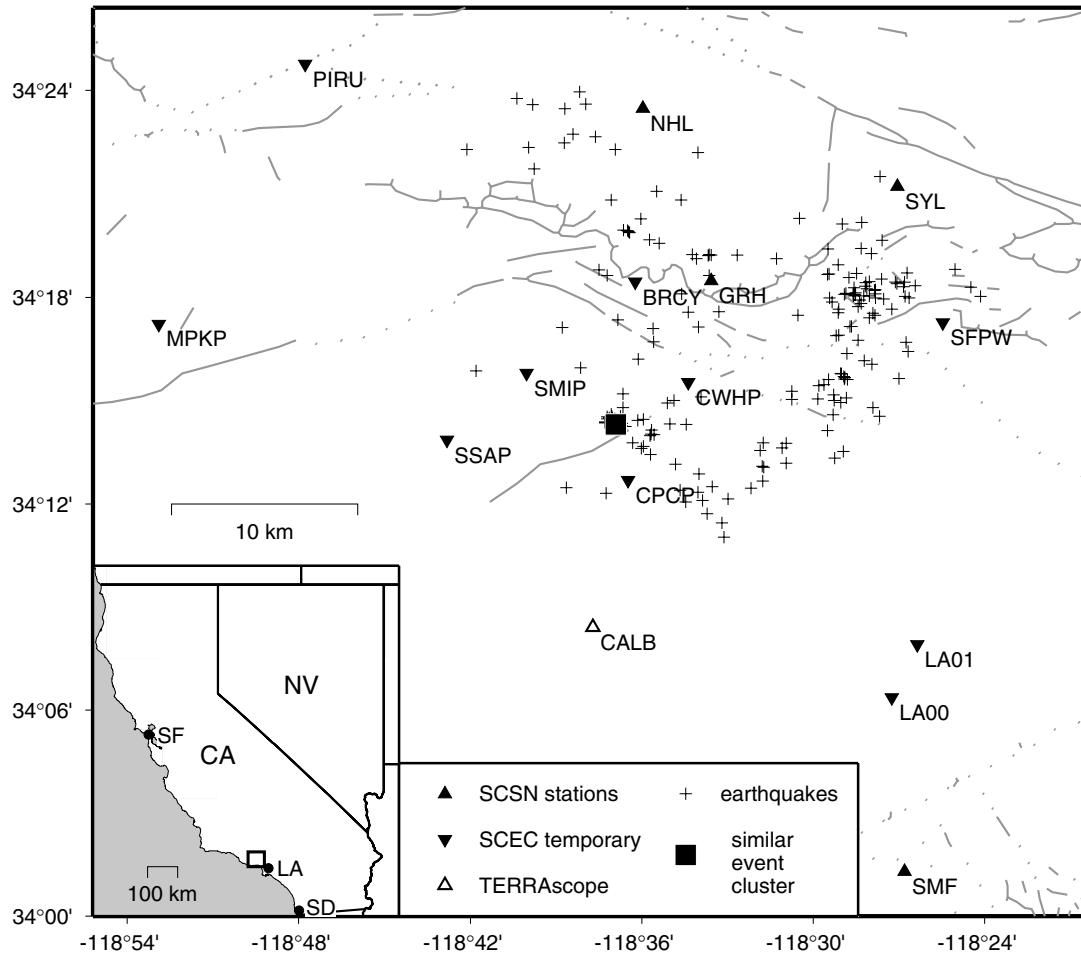
Figure 1. Map of the Northridge region, California. Crosses mark the epicenters of 203 earthquakes used in this study, and the square indicates the location of the similar event cluster. Stations are marked by triangles. Open triangle, TERRAScope permanent broadband station; upright filled triangles, short-period permanent SCSN stations; inverted filled triangles, short-period SCEC portable stations. Gray lines indicate mapped fault traces from Jennings (1975). Box in inset map shows location. CA, California; NV, Nevada; LA, Los Angeles; SD, San Diego; SF, San Francisco.
