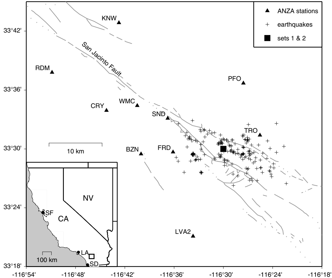
Figure 6. Map of the Anza region, California. Crosses mark the 197 events used, and the square indicates the location of the 42 colocated events of sets 1 and 2. Stations of the broadband Anza seismic network are marked by triangles. Faults from Jennings (1975) as gray lines.
