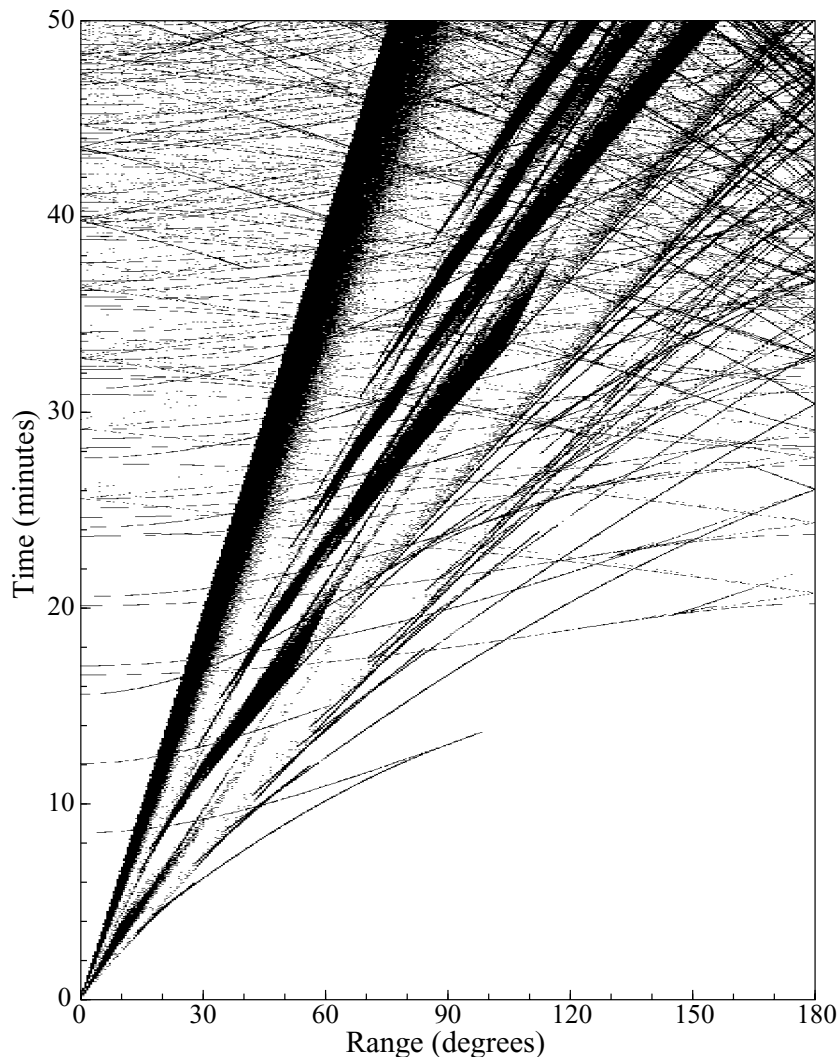
Figure 10. Theoretical traveltimes curves predicted using the seismic phonon method. Most of these have amplitudes too small to see in real data.
