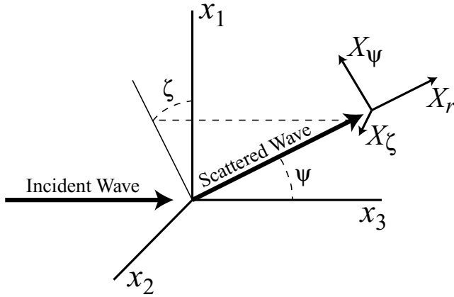
Figure 5. The ray-centred coordinate system used in the scattering equations. The incident ray is in the x_3 direction. For S waves the initial polarization is in the x_1 direction. The scattered ray direction is defined by the angles \psi and \zeta . The scattered ray polarization is defined by X_r , X_\psi and X_\zeta .
