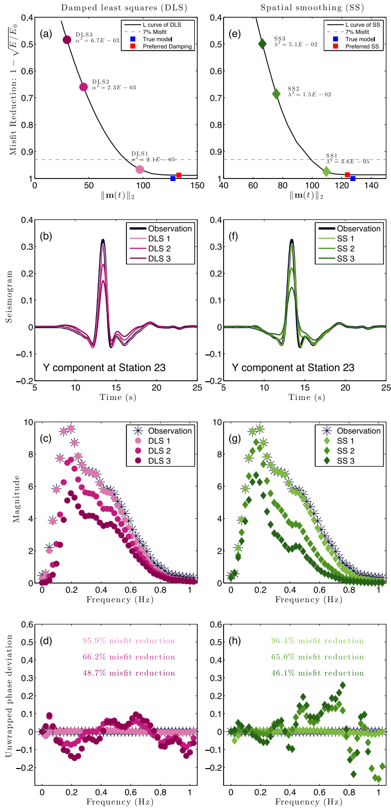
Figure 13. Regularization strength trade-off ('L') curves for inversion with SIV1 provided data (see text). Panel layout is similar to Fig. 5, only the grey dashed line represents 7 per cent misfit level.
