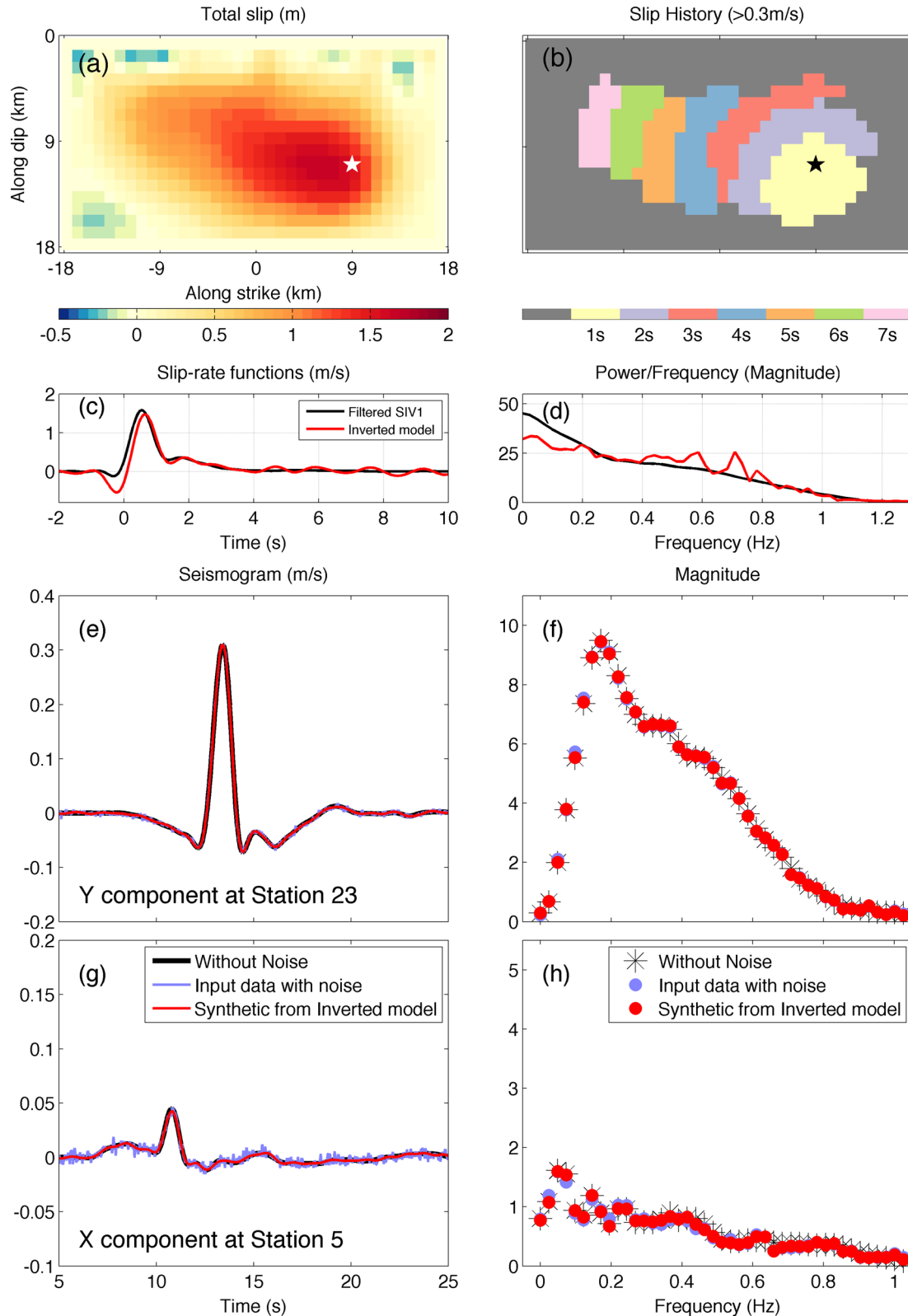
Figure 15. Inverted source model from data with Gaussian noise ( \text{SNR}_1 ). (a) Total slip; (b) slip history; (c) slip-rate function at hypocentre; (d) spectrum of the slip-rate function; (e) seismograms with the largest peak amplitude; (f) spectra of the seismograms (e); (g) seismogram with the median peak amplitude; (h) spectra of the seismograms (g).
