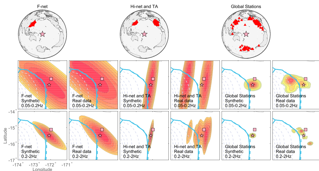
Figure 7. Comparison of theoretical resolving power and time-integrated back-projection results from two frequency bands ((top) LF; (bottom) HF) for the Tonga-Samoa earthquake obtained from F-net, a combined array (Hi-net and TA), and the global stations.
