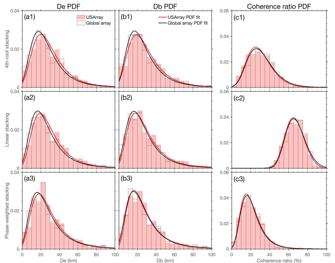
Figure 13. Distributions of D_e , D_b , and coherence ratios at 0.3–1 Hz. The fitted probability density functions (PDF) follow generalized extreme value (GEV) distributions, whose parameters are listed in Table 1.
