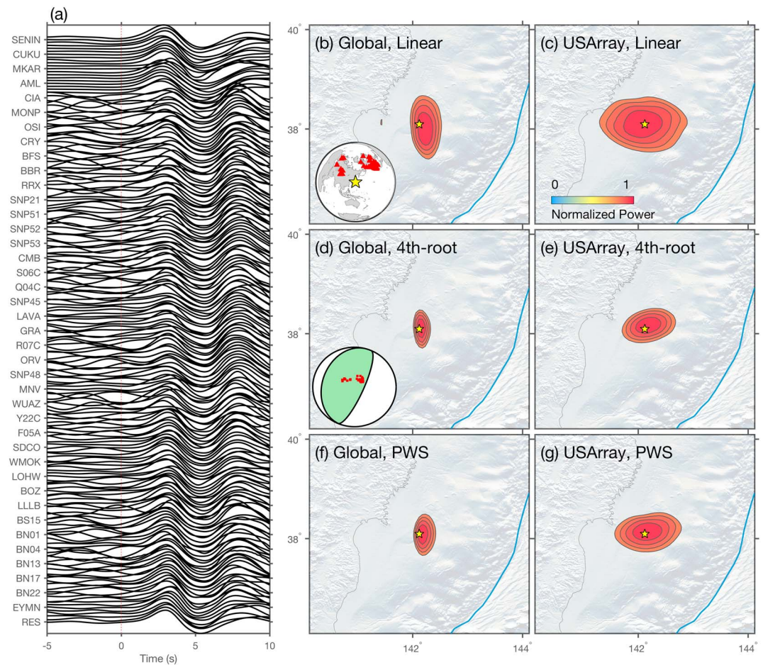
Figure 3. Backprojection results for Event 4 (Figure 1) with self-aligned time calibrations (0.05–0.3 Hz, 80% energy contour). (a) Velocity records sorted with azimuth. (b, d, and f) Integrated backprojection result of the first 20 s with linear, fourth-root stacking, and phase-weighted stacking (PWS). Station map (Figure 3b). Lower hemisphere P wave polarities of the stations, the focal mechanism is for Event 4 (2 December 2005 M_w 6.5) (Figure 3d). (c, e, and g) Similar to Figures 3b, 3d, and 3f, but only using stations within the azimuthal range from 0° to 90°.
