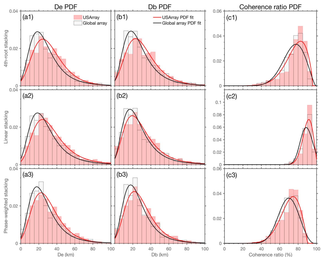
Figure 12. Distributions of D_e , D_b , and coherence ratios at 0.05–0.3 Hz. The fitted probability density functions (PDF) follow generalized extreme value (GEV) distributions, which parameters are listed in Table 1.
